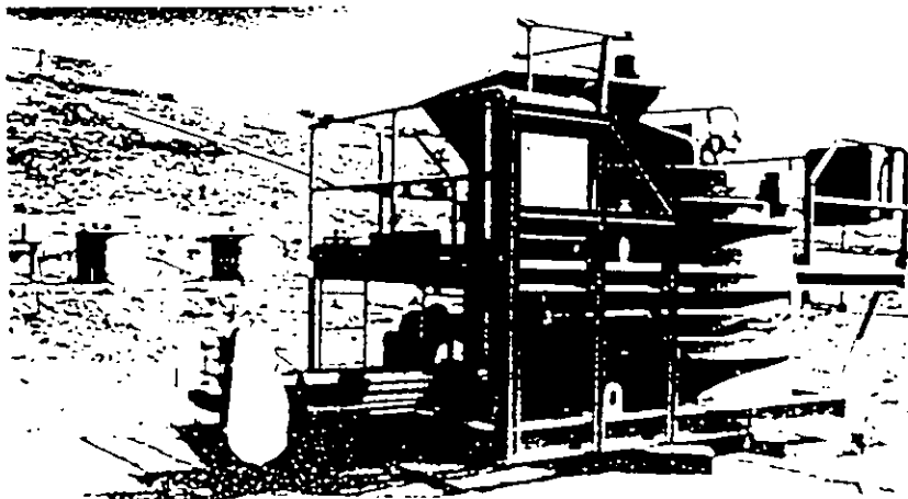
A mechanical composter, approved for use with explosives-contaminated soil, has been procured and will be used in comparison tests with other composting methods.
